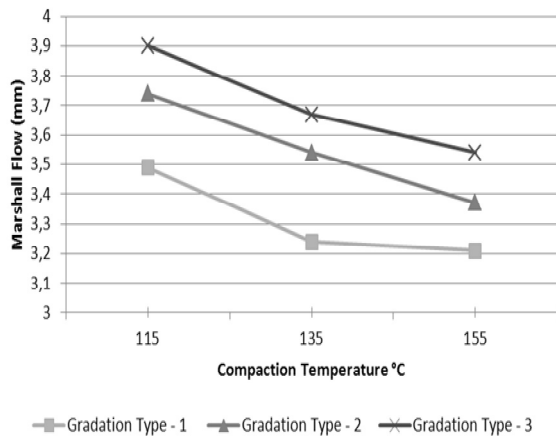
Fig. 13 Relationship of Compaction Temperature Versus Marshal Flow of Asphalt Concrete Mixture Being Soaked in Water for 1 Day at 60°C
