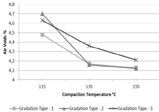
Fig. 3. Relationship of Compaction Temperature Versus Percent Air Voids in Asphalt Concrete Mixture
