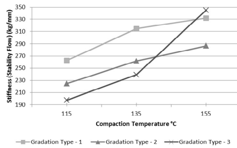
Fig. 21 Relationship of Compaction Temperature Versus Stiffness of Dry Asphalt Concrete Mixture Being Soaked in Water for 2 Days at 60°
