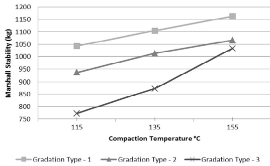
Fig. 7 Relationship of Compaction Temperature Versus Marshal Stability of Asphalt Concrete Mixture Being Soaked in Water for 2 Days at 60°C
