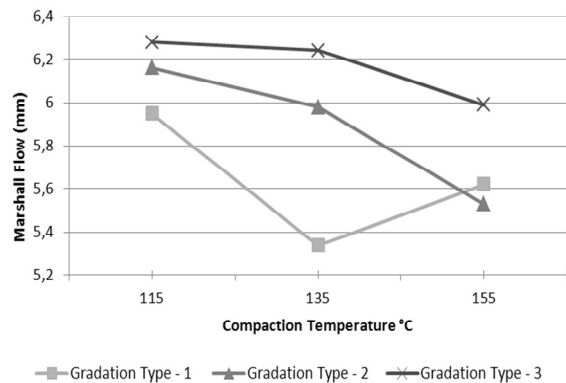
Fig. 18 Relationship of Compaction Temperature Versus Marshal Flow of Asphalt Concrete Mixture Being Soaked in Water for 28 Days at 60°C
