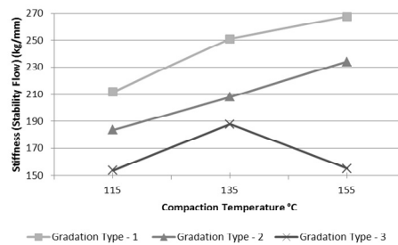
Fig. 22 Relationship of Compaction Temperature Versus Stiffness of Dry Asphalt Concrete Mixture Being Soaked in Water for 4 Days at 60°
