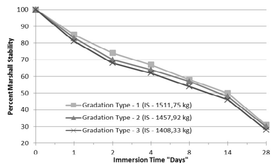
Fig. 27 Durability Curves for Aggregate Gradation Types, Using Marshall Stability Criterion, At Compaction Temperature 135°C (IS – Initial Stability)
