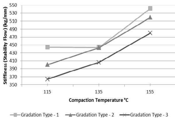
Fig. 19 Relationship of Compaction Temperature Versus Stiffness of Dry Asphalt Concrete Mixture
