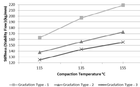
Fig. 23 Relationship of Compaction Temperature Versus Stiffness of Dry Asphalt Concrete Mixture Being Soaked in Water for 8 Days at 60°C
