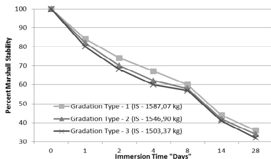
Fig. 28 Durability Curves for Aggregate Gradation Types, Using Marshall stability Criterion, At Compaction Temperature 155°C (IS – Initial Stability)
