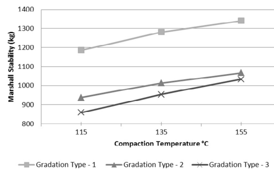
Fig. 6 Relationship of Compaction Temperature Versus Marshall Stability of Asphalt Concrete Mixture Being Soaked in Water for 1 Day at 60°C
