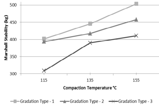
Fig. 11 Relationship of Compaction Temperature Versus Marshal Stability of Asphalt Concrete Mixture Being Soaked in Water for 28 Days at 60°C
