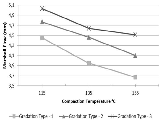
Fig. 15 Relationship of Compaction Temperature Versus Marshal Flow of Asphalt Concrete Mixture Being Soaked in Water for 4 Days at 60°C
