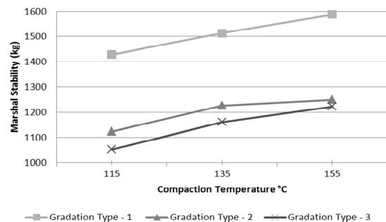
Fig. 5 Relationship of Compaction Temperature Versus Marshall Stability Dry Asphalt Concrete Mixture
