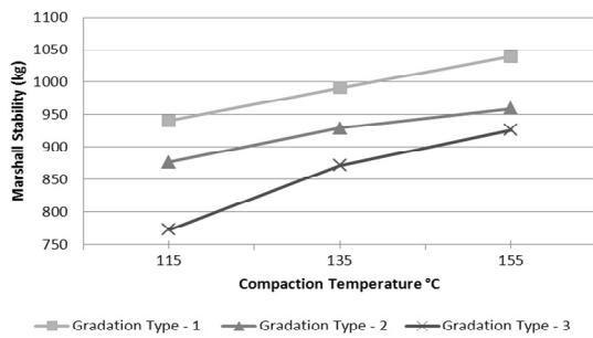
Fig. 8 Relationship of Compaction Temperature Versus Marshal Stability of Asphalt Concrete Mixture Being Soaked in Water for 4 Days at 60°C
