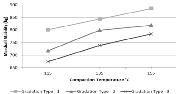
Fig. 9 Relationship of Compaction Temperature Versus Marshal Stability of Asphalt Concrete Mixture Being Soaked in Water for 8 Days at 60°C
