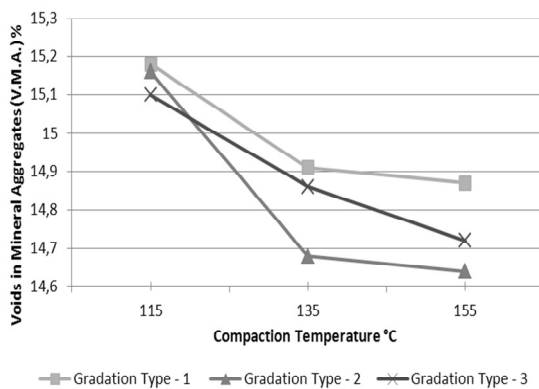
Fig. 4 Relationship of Compaction Temperature Versus Percent Voids in Mineral Aggregates (V.M.A.) %
