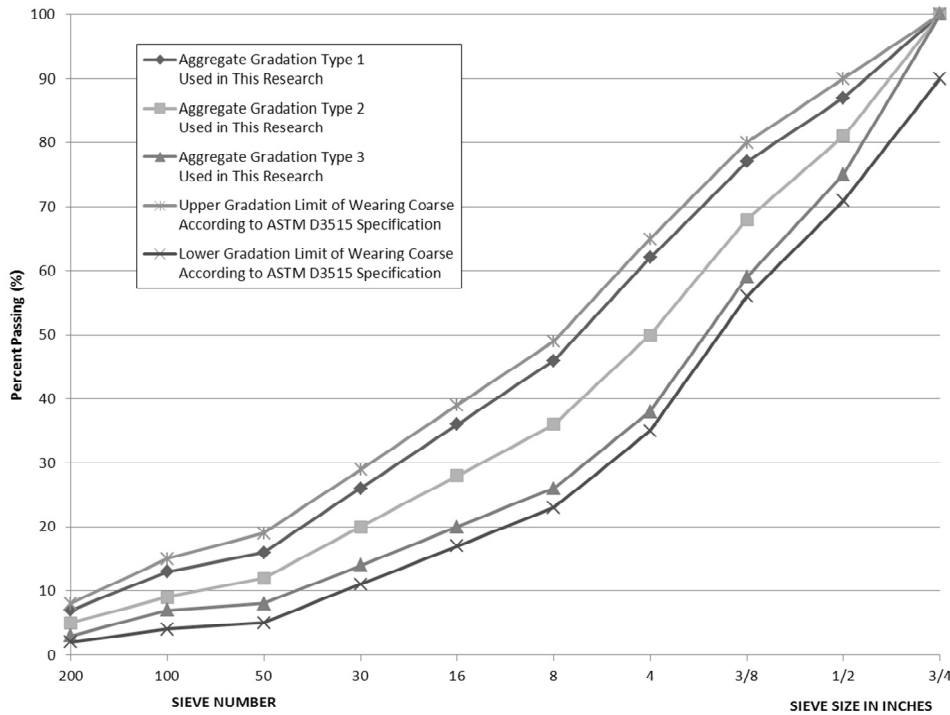
Fig. 1. Gradation Limits of Wearing Aggregate According to ASTM D3515 and Gradation Types used in This Research
