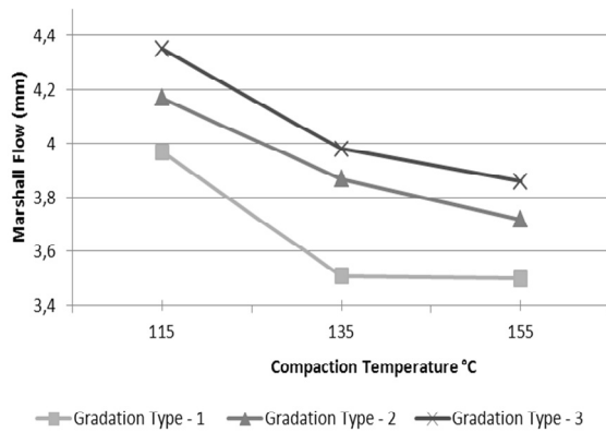
Fig. 14 Relationship of Compaction Temperature Versus Marshal Flow of Asphalt Concrete Mixture Being Soaked in Water for 2 Days at 60°C
