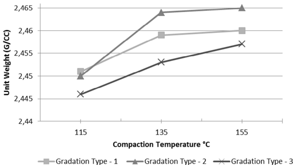
Fig. 2. Relationship of Compaction Temperature Versus Unit Weight of Asphalt Concrete Mixture
