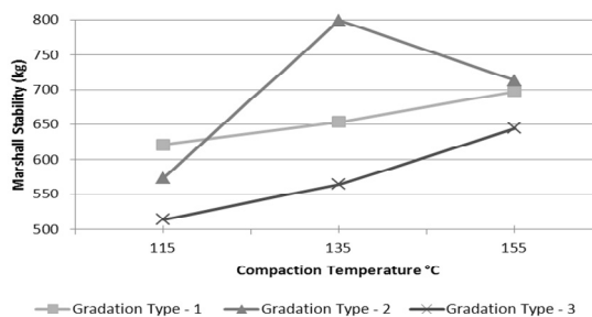
Fig. 10 Relationship of Compaction Temperature Versus Marshal Stability of Asphalt Concrete Mixture Being Soaked in Water for 14 Days at 60°C
