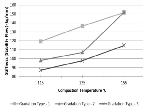
Fig. 24 Relationship of Compaction Temperature Versus Stiffness of Dry Asphalt Concrete Mixture Being Soaked in Water for 14 Days at 60°C
