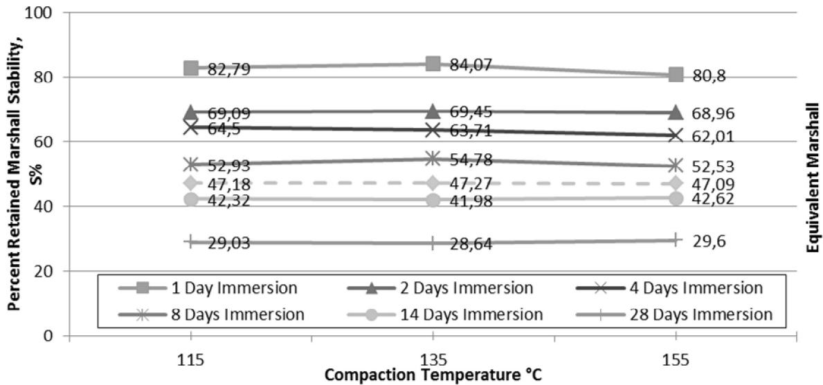
Fig. 30 The Effect of Compaction Temperature on the Durability Potential of the Mixture Type - 2 at Different Periods of Immersion, Using Marshall Stability Criterion
