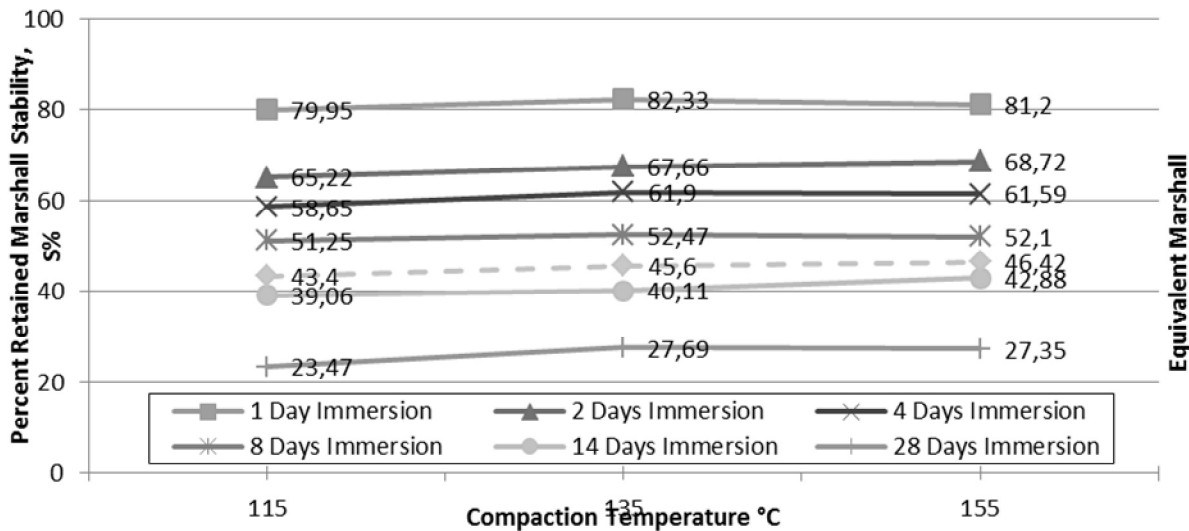
Fig. 31 The Effect of Compaction Temperature on the Durability Potential of the Mixture Type - 3 at Different Periods of Immersion, Using Marshall Stability Criterion
