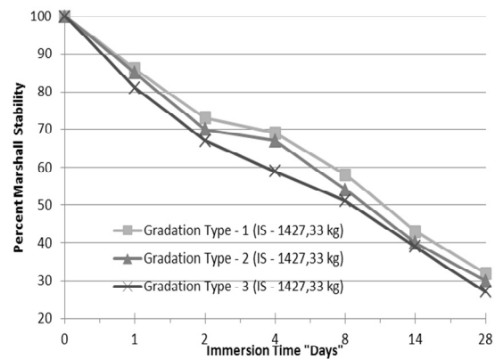
Fig. 26 Durability Curves for Aggregate Gradation Types, Using Marshall Stability Criterion, At Compaction Temperature 115°C (IS – Initial Stability)
