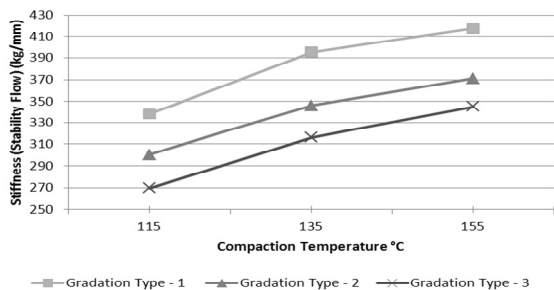
Fig. 20 Relationship of Compaction Temperature Versus Stiffness of Dry Asphalt Concrete Mixture Being Soaked in Water for 1 Day at 60°C
