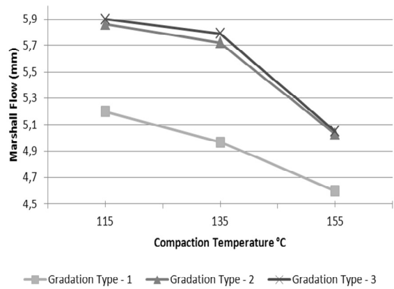
Fig. 17 Relationship of Compaction Temperature Versus Marshal Flow of Asphalt Concrete Mixture Being Soaked in Water for 14 Days at 60°C
