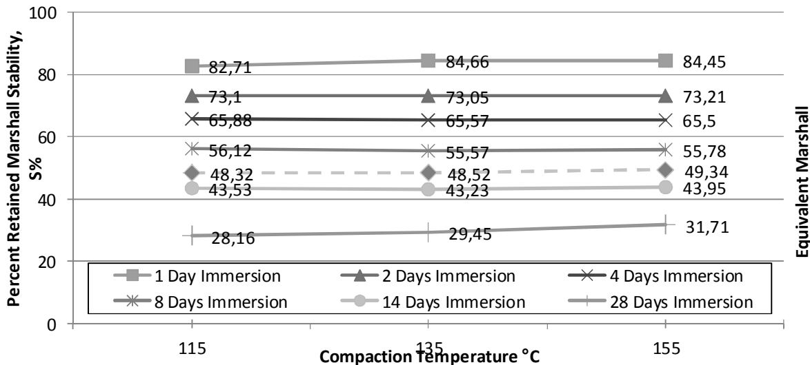
Fig. 29 The Effect of Compaction Temperature on the Durability Potential of the Mixture Type - 1 at Different Periods of Immersion, Using Marshall Stability Criterion
