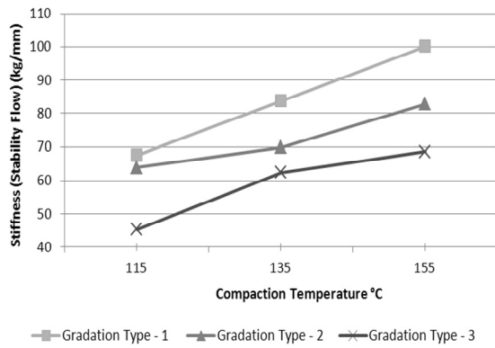
Fig. 25 Relationship of Compaction Temperature Versus Stiffness of Dry Asphalt Concrete Mixture Being Soaked in Water for 28 Days at 60°C
