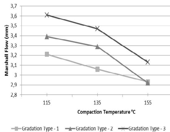
Fig. 12 Relationship of Compaction Temperature Versus Marshal Flow of Dry Asphalt Concrete Mixture
