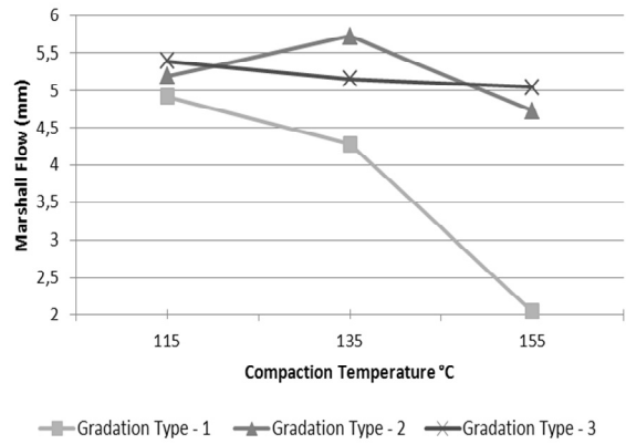
Fig. 16 Relationship of Compaction Temperature Versus Marshal Flow of Asphalt Concrete Mixture Being Soaked in Water for 8 Days at 60°C
