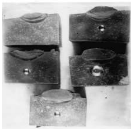
Fig. 3. Macrostructure of Weld Joints
