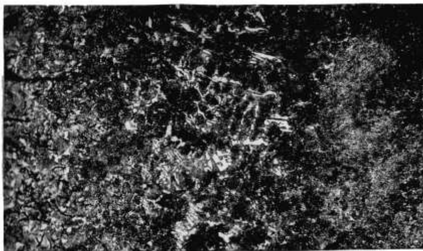
Fig. 5. Microstructure of cast iron-steel melting zone, \times 450
