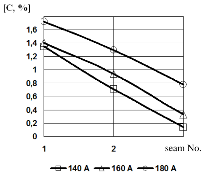
Fig. 6. Dependence of the carbon content in the weld metal on the current strength at reverse polarity welding
