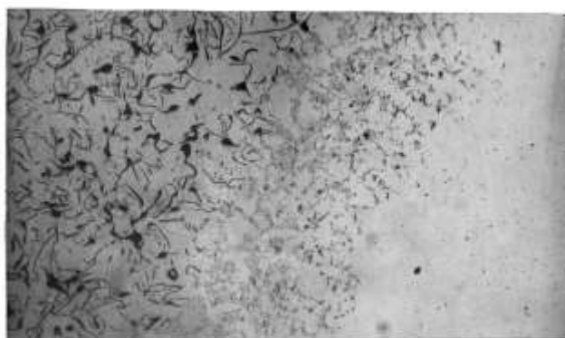
Fig. 4. Melting zone of cast iron-steel, \times 100 , not damaged
