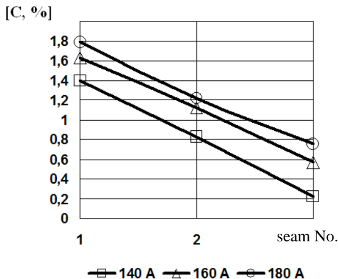
Fig.7. Dependence of carbon content in the weld metal on the current strength at direct polarity welding
