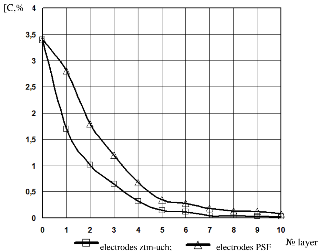
Fig. 1. Dependence of carbon content in metal on seam height
