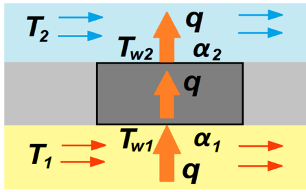
Fig. 3. The design scheme of the cooled engine element in the steady state heat condition
